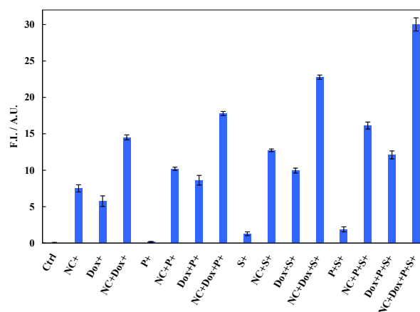
Figure 7: F.L.s of MCF-7 cells as indicators of intracellular ROS levels upon treatment with laser light (P + ), US waves (S + ), laser light/US waves (P + S + ), Au-PoAP NC of 5 μg mL -1 (NC + ), laser light/US waves (P + S + ), Au-PoAP NC of 5 μg mL -1 with doxorubicin of 0.58 μg mL -1 (NC + Dox + ), Au-PoAP NC of 5 μg mL -1 upon PTT (NC + P + ), SDT (NC + S + ) and PTT/SDT (NC + P + S + ), doxorubicin of 0.58 μg mL -1 upon PTT (Dox + P + ), SDT (Dox + S + ) and PTT/SDT (Dox + P + S + ), and Au-PoAP NC of 5 μg mL -1 with doxorubicin of 0.58 μg mL -1 upon PTT (NC + Dox + P + ), SDT (NC + Dox + S + ) and PTT/SDT (NC + Dox + P + S + )
